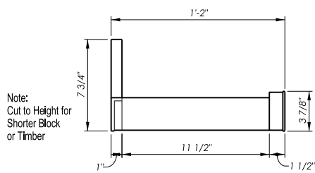
Wall Drain Pro Detail - Side View
