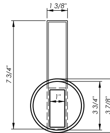
Wall Drain Pro Detail - End View
