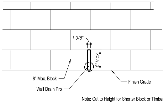
Wall Elevation
