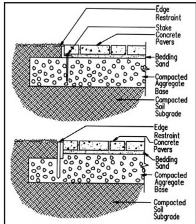
Figure 6. Aluminum and steel edging.
