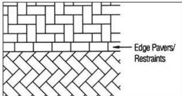
Figure 1. Change in laying pattern direction.
