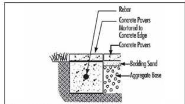
Figure 10. Submerged concrete edge.
