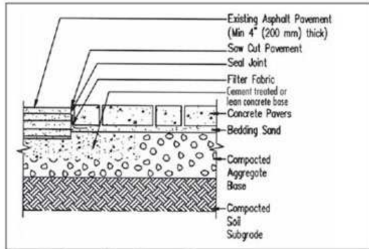
Figure 14. Crosswalk in existing asphalt pavement.
