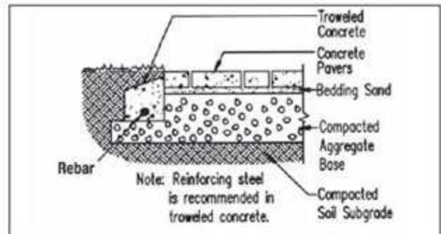
Figure 9. Troweled concrete edges.
