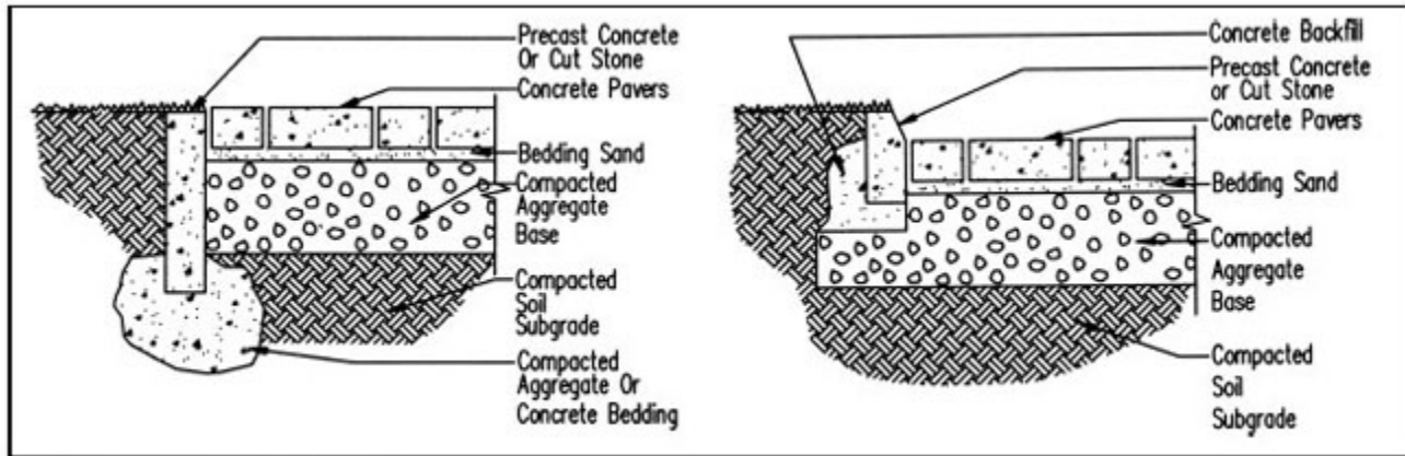
Figure 4. Precast concrete/cut stone.
