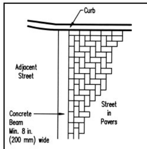
Figure 12. Concrete beam.
