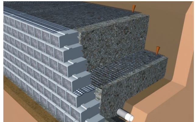
Example of segmental retaining wall reinforcement.
