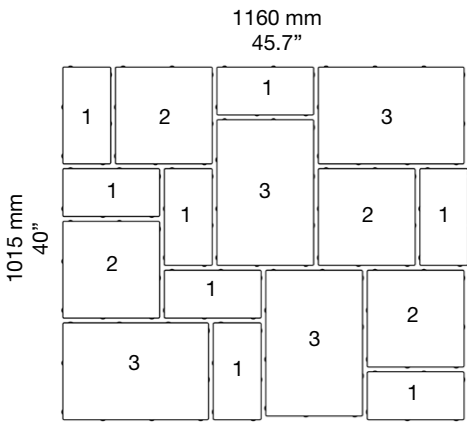
Pallet Layer Pattern River Rock 1 (8 Pavers); River Rock 2 (4 Pavers) River Rock 3 (4 Pavers)
